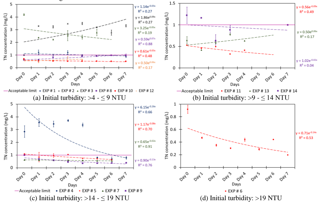
Figure 6: Removal trends of TN for different experiments carried out in different turbidity ranges
