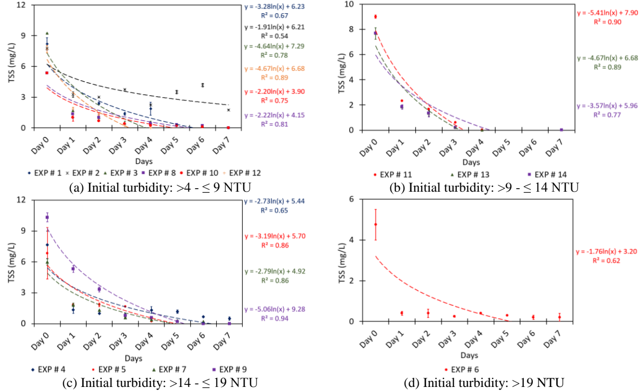
Figure 4: Removal trend of TSS for different experiments carried out in different turbidity ranges
