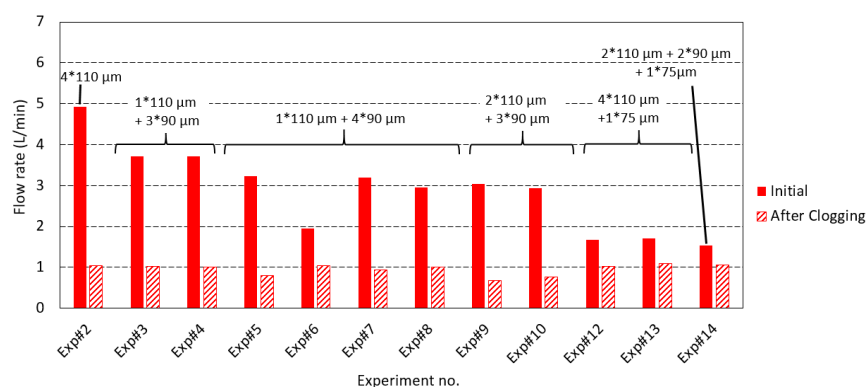
Figure 8: Flow rate as a function of filter
