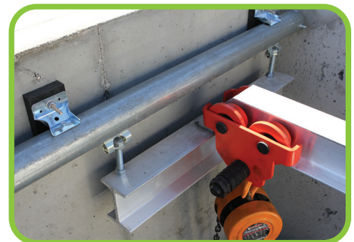
Trolley System
